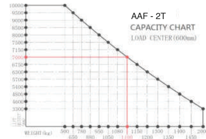
Capacity Chart AAF - 2T
