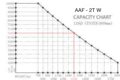
Capacity Chart -AAF - 2T W
