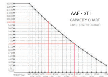
Capacity Chart- AAF - 2T H
